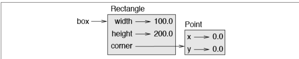
Figure 15-2. Object diagram.
