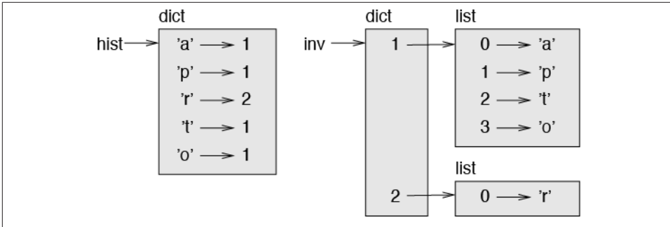
Figure 11-1. State diagram.
